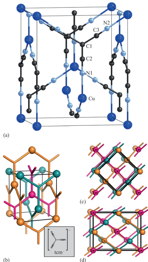
Fig. 3 (a) Representation of the crystal structure of \beta -Cu(tcm), viewed with the tetragonal c axis oriented vertically. Thermal ellipsoids are represented at 50% probability. (b) Topological representation of the same framework, where Cu atoms are shown as large spheres, tcm moieties in stick representation, and the unit cell in black. The three mutually-interpenetrating (10,3)- b frameworks are coloured differently. The inset shows the chemical structure of the tricyanomethanide anion. (c) The same framework, viewed slightly away from c , illustrating its square wine-rack geometry with \theta = 90^\circ . (d) The low-temperature \alpha -Cu(tcm) phase—shown here in terms of the structural model determined using powder X-ray diffraction data collected at 20 K—has the same network connectivity, but the loss of tetragonal symmetry allows \theta to deviate from 90^\circ . The Fdd2 unit cell, shown here in black, has twice the volume of the I4_1md cell of \beta -Cu(tcm).
