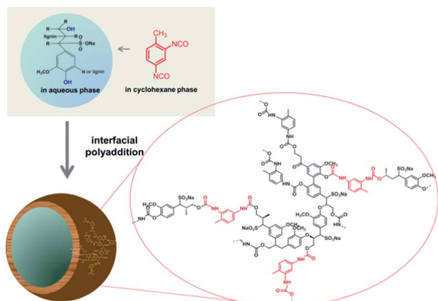
Scheme 1 Synthetic protocol for the generation of hollow lignin nanocontainers by inverse miniemulsion.
