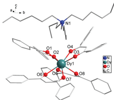
Fig. 1 Partially labelled molecular structure of [\text{Hex}_4\text{N}][\text{Dy}(\text{DBM})_4] , 1 . Colour code: Dy (teal), O (red), N (blue), C (grey). H atoms and disordered atoms were omitted for clarity.
