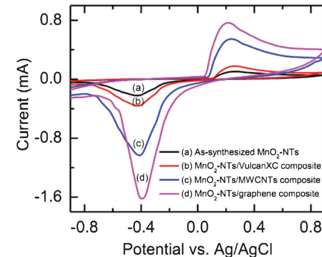
Fig. 3 Cyclic voltammograms of (a) the as-synthesized MnO 2 -NTs, (b) MnO 2 -NTs/Vulcan, (c) MnO 2 -NTs/MWCNTs, and (d) MnO 2 -NTs/graphene composites in air saturated 1 M KCl solution.
