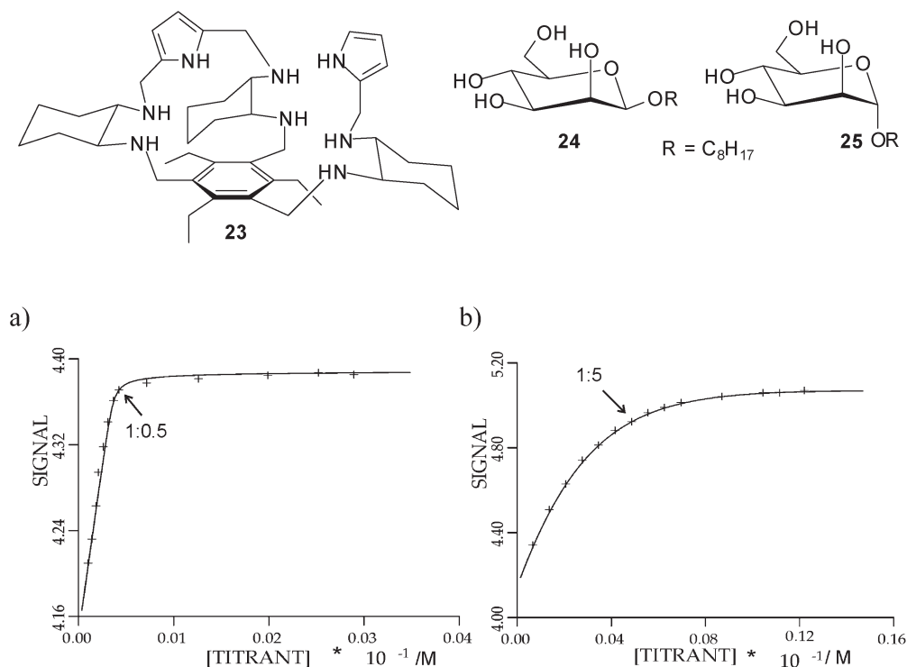
Fig. 6 Plot of the observed ( \times ) and calculated ( - ) chemical shifts of the NH resonances of 27 (1.02 mM) as a function of added \beta -maltoside 28 (a) or \beta -glucopyranoside 2a (b). The [receptor]:[sugar] ratio is marked. 24
