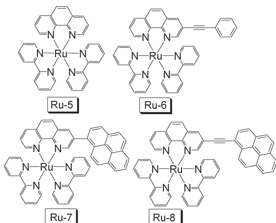
Fig. 4 Chemical structures of the sensitizer Ru II complexes Ru-5 ~ Ru-8 . Note the complexes are dicationic and the [PF 6 ] - ions are omitted for clarity. The compounds are from ref. 16.
