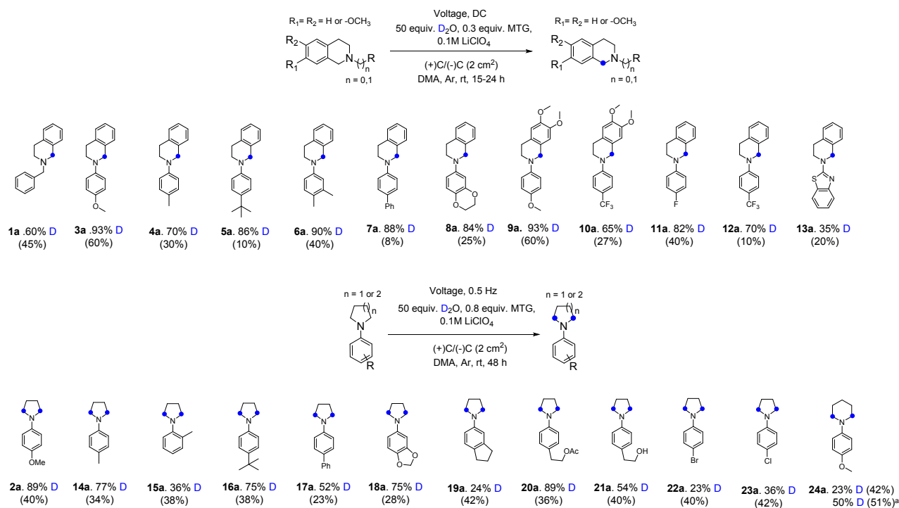
Fig. 4. Substrate scope of electrochemical HIE reaction. a Reaction was conducted at 50 Hz. D incorporation was determined by 1 H NMR peak integration relative to an unlabeled compound. All isolated yields were provided in parentheses. The experimental voltage for each substrate is provided in SI.
