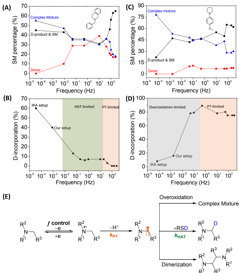
Fig. 2. f -dependent of product distribution in terms of starting material (SM) conversion and D incorporation for (A)-(B) 1 and (C)-(D) 2 . (E) Illustration of the f -controlled pathways towards forming D-substituted amine, dimer, and overoxidized complex mixture.
