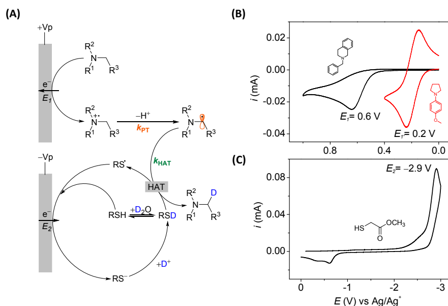
Fig. 1. (A) Proposed mechanism for AC-driven HIE of amines. Cyclic voltammograms of (B) 1 (black), 2 (red) and (C) methyl thioglycolate (MTG) in N,N' -dimethylacetamide (DMA) containing 0.1 M LiClO 4 . Scan rate: 0.1 V/s.
