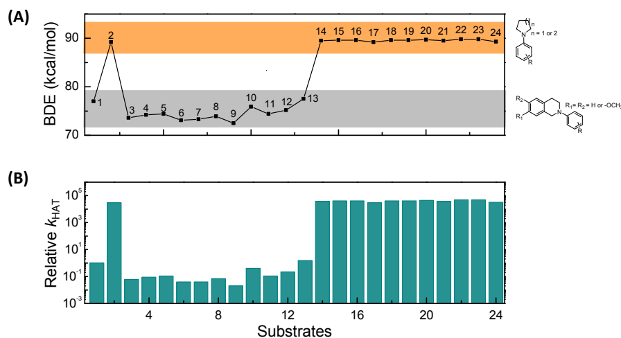
Fig. 3. (A) Calculated BDE values and (B) predicted relative HAT rate of \alpha -amino C(sp 3 )-H sites for different substituted tetrahydroisoquinolines ( 1 , 3-13 ), pyrrolidines ( 2 , 14-23 ) and piperidine ( 24 ).
