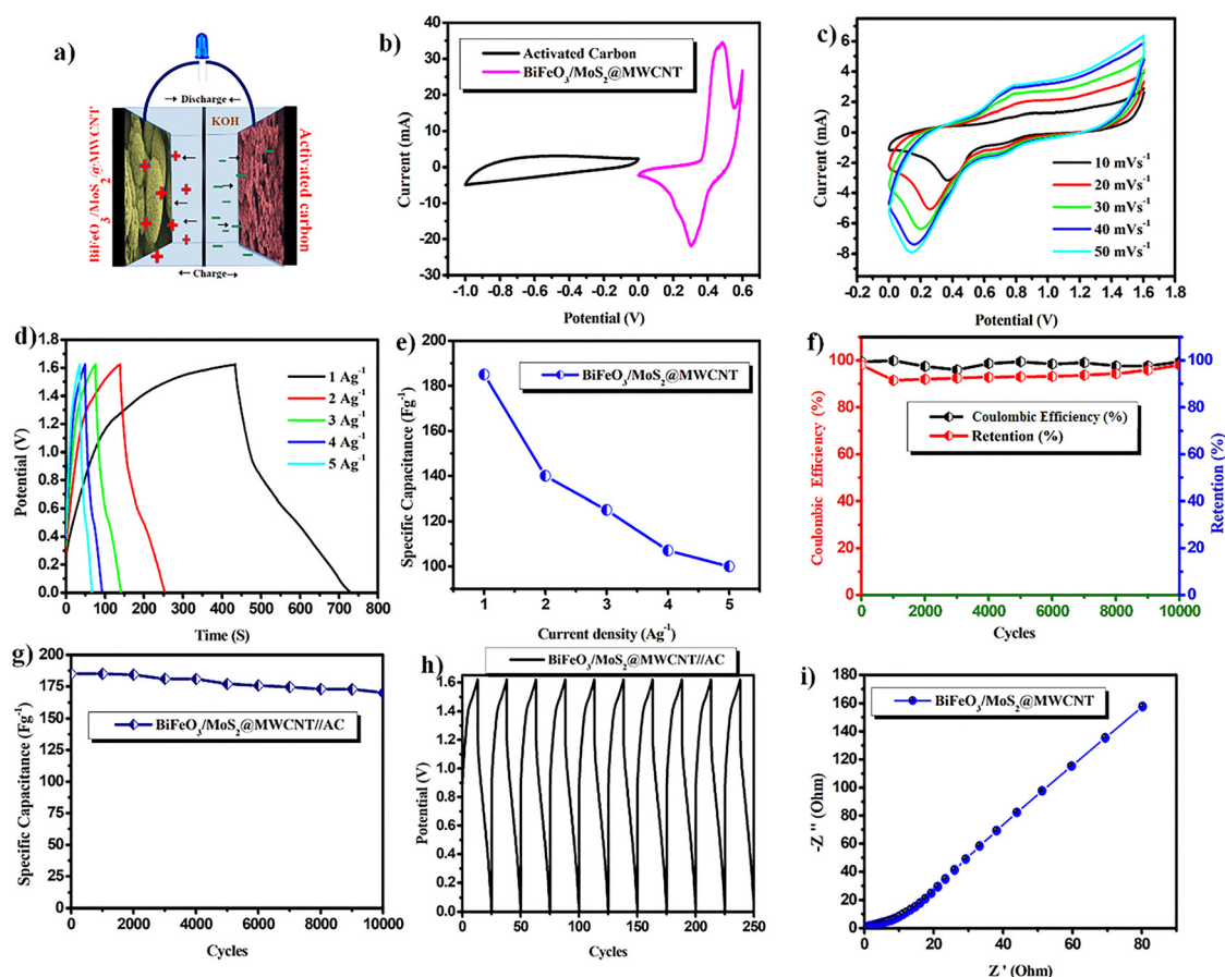
Fig. 7 (a) Schematic representation of the assembled \text{BiFeO}_3/\text{MoS}_2@\text{MWCNT} // \text{AC} asymmetric supercapacitor; (b) comparative cyclic voltammetry curves of \text{BiFeO}_3/\text{MoS}_2@\text{MWCNT} and AC electrodes at 10\ \text{mV s}^{-1} ; (c) CV profiles of the full asymmetric device at various scan rates; (d) Galvanostatic charge–discharge profiles of the ASC device; (e) C_s at different current densities; (f) capacitance retention and Coulombic efficiency over 10 000 cycles; (g) specific capacitance evolution during the cycling testing; (h) charge–discharge profiles for the initial 250 cycles; (i) electrochemical impedance spectroscopy analysis of the ASC device.
