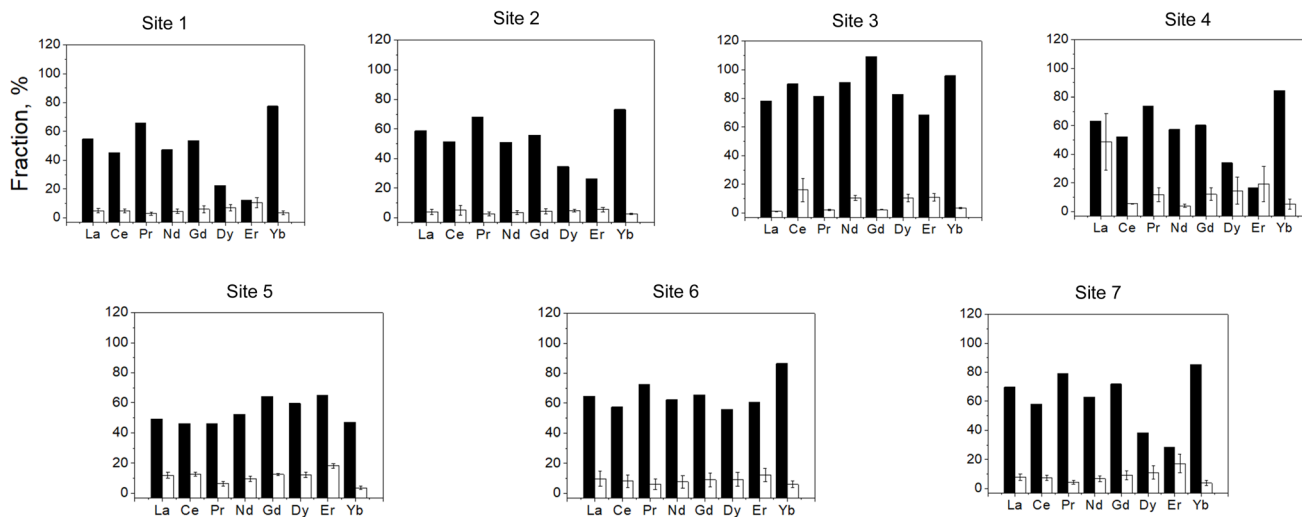
Fig. 4 Filtered (FF) and Labile fractions (LF) for samples collected during the wet season as % of total fraction. FF = black bar. LF = white bar. The bar represent standard deviation of measurement performed by DGT.
