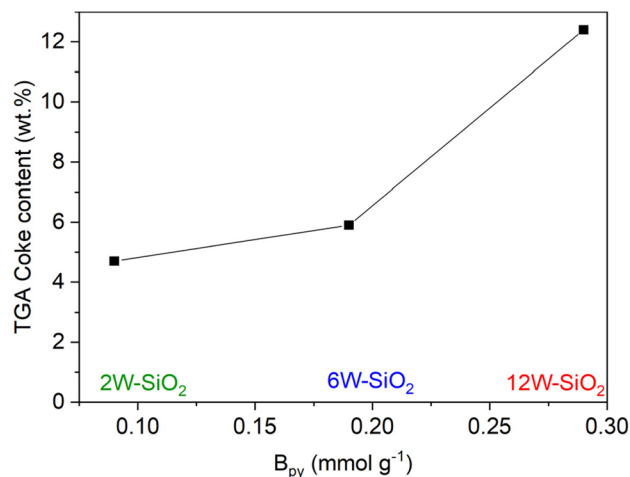
Fig. 13 Correlation between the number of Brønsted acid sites ( B_{py} ) and coke content in the spent catalysts.
