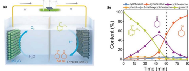
Fig. 19 (a) Schematic representation of the ECH of guaiacol into a KA-oil mixture using PtNiB/CMK-3 as the cathode and IrO 2 /C as the anode and (b) concentration profile of guaiacol and hydrogenated products over PtNiB/CMK-3. Adapted from ref. 125 with permission from Adv. Funct. Mater. , 2019, 29, 1807651. Copyright 2019, Wiley-VCH.
