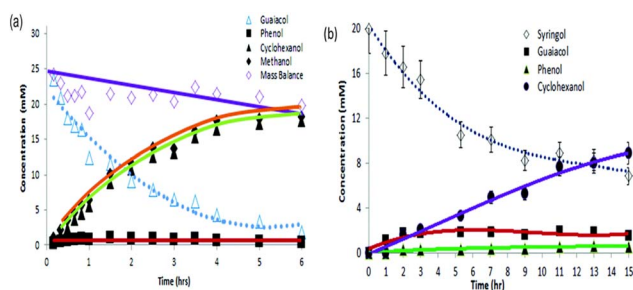
Fig. 20 (a) ECH of guaiacol to cyclohexanol at a current density of 8 \text{ mA cm}^{-2} and a temperature of 75 \text{ °C} in a 0.1 M potassium borate buffer; (b) ECH of syringol in a 0.1 M potassium borate buffer containing 0.5 mM cetyltrimethylammonium bromide (CTAB) at 75 \text{ °C} . Adapted from ref. 124 with permission from Green Chem. , 2015, 17, 601–609. Copyright 2015, Royal Society of Chemistry.
