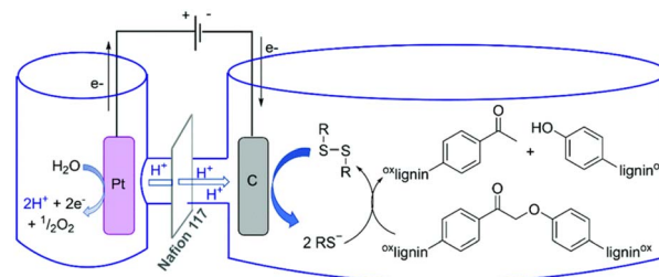
Fig. 28 Potential schematic mechanism of lignin deconstruction in a thio-assisted electrolytic system. Reproduced from ref. 113 with permission from Green Chem. , 2021, 23, 412–421. Copyright 2021, Royal Society of Chemistry.
