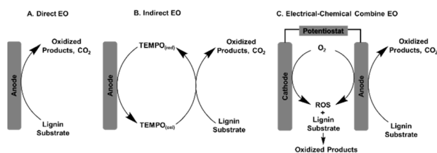
Fig. 4 Typical routes of lignin electrochemical oxidation (EO): (A) direct oxidation, (B) indirect oxidation, and (C) electrical-chemical combined oxidation. Reproduced from ref. 58 with permission from ChemSusChem. , 2020, 13, 4318–4343. Copyright 2020, John Wiley and Sons.
