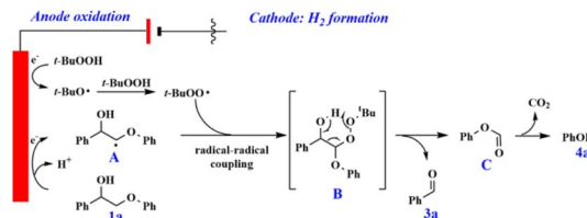
Fig. 9 Possible reaction pathway for the cleavage of the \text{C}_\alpha\text{--C}_\beta bond in the \beta\text{-O-4} lignin model compound. Reproduced from ref. 94 with permission from ACS Sustain. Chem. Eng., 2021, 9, 1932–1940. Copyright 2021, American Chemical Society.
