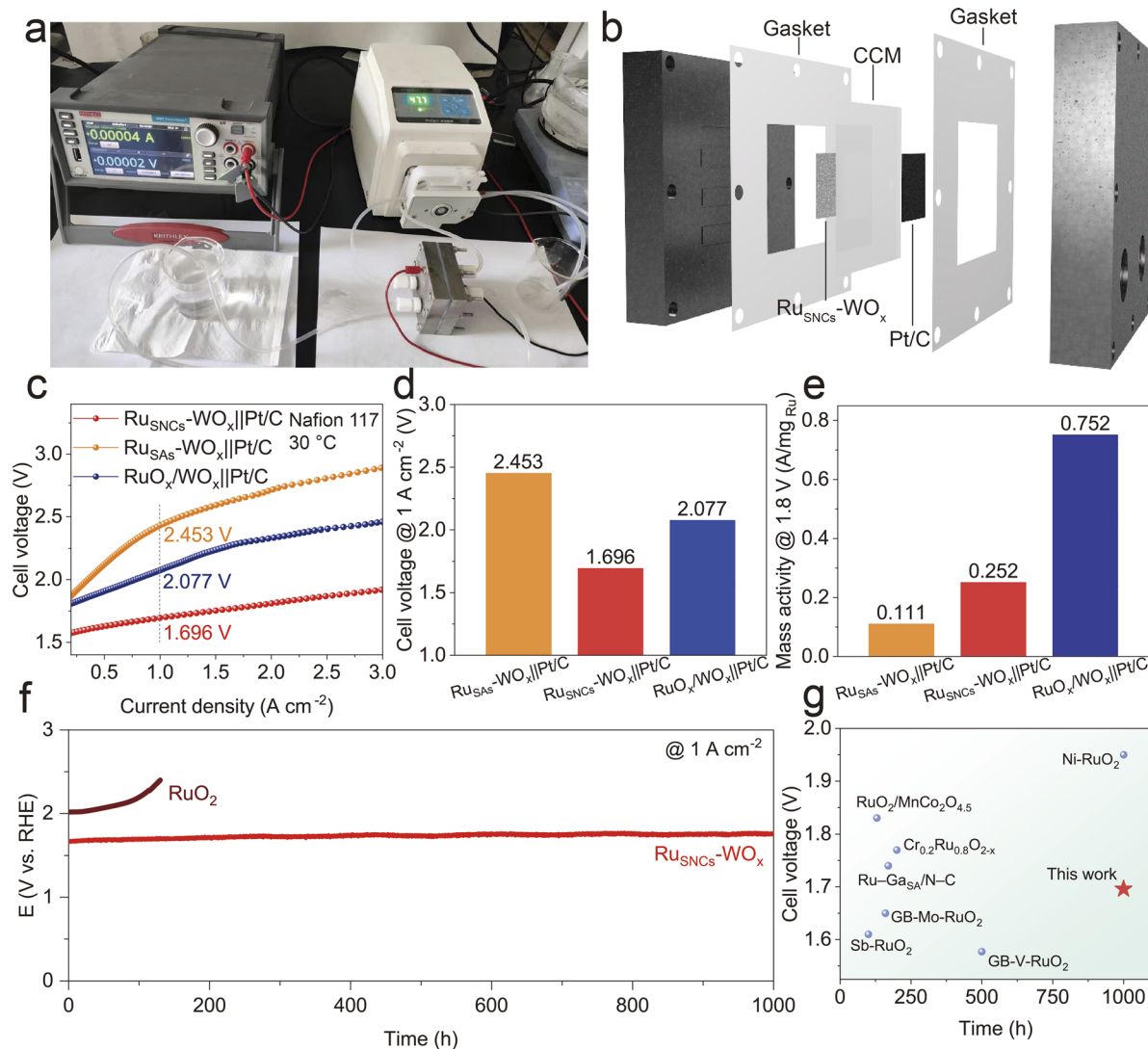
Fig. 6 (a) PEMWE device. (b) Schematic of the PEMWE cell. (c) The polarization curves of PEMWE obtained using \text{Ru}_{\text{SAs}}\text{-WO}_x , \text{Ru}_{\text{SNCs}}\text{-WO}_x and \text{RuO}_x/\text{WO}_x as the anode catalysts at 30 °C with a Nafion 117 proton exchange membrane. (d) Comparison of overpotentials for \text{Ru}_{\text{SNCs}}\text{-WO}_x\|\text{Pt/C} , \text{Ru}_{\text{SAs}}\text{-WO}_x\|\text{Pt/C} and \text{RuO}_x/\text{WO}_x\|\text{Pt/C} at a current density of 1 \text{A cm}^{-2} . (e) Mass activity of \text{Ru}_{\text{SNCs}}\text{-WO}_x\|\text{Pt/C} , \text{Ru}_{\text{SAs}}\text{-WO}_x\|\text{Pt/C} and \text{RuO}_x/\text{WO}_x\|\text{Pt/C} based on the mass of Ru. (f) Chronopotentiometry of PEMWE based on \text{Ru}_{\text{SNCs}}\text{-WO}_x\|\text{Pt/C} and \text{RuO}_2\|\text{Pt/C} . (g) Comparison of the stability of PEMWE using \text{Ru}_{\text{SNCs}}\text{-WO}_x as well as other reported \text{RuO}_2 -based anode catalysts.
