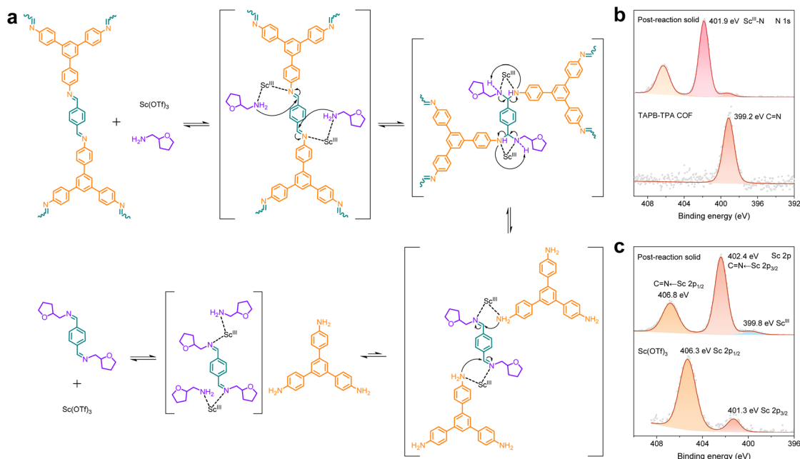
Fig. 6 (a) Schematic illustration for the \text{Sc(OTf)}_3 -catalyzed transamination mechanism. (b) High-resolution XPS N 1s spectra of TAPB-TPA COF and the post-reaction solid. (c) High-resolution XPS Sc 2p spectra of \text{Sc(OTf)}_3 and the post-reaction solid.
