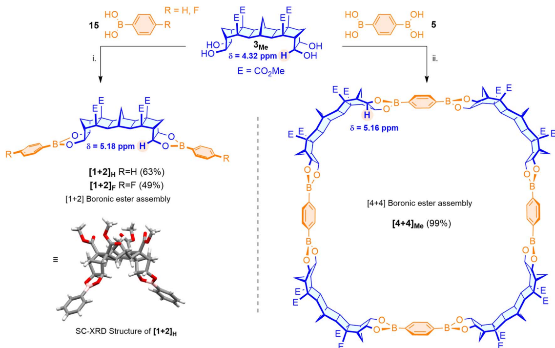
Scheme 2 Synthesis of [1 + 2] assemblies and [4 + 4] macrocycle. (i) EtOH, 130 °C, 5 min, \mu w. (ii) CHCl 3 , 100 °C, 12 h.
