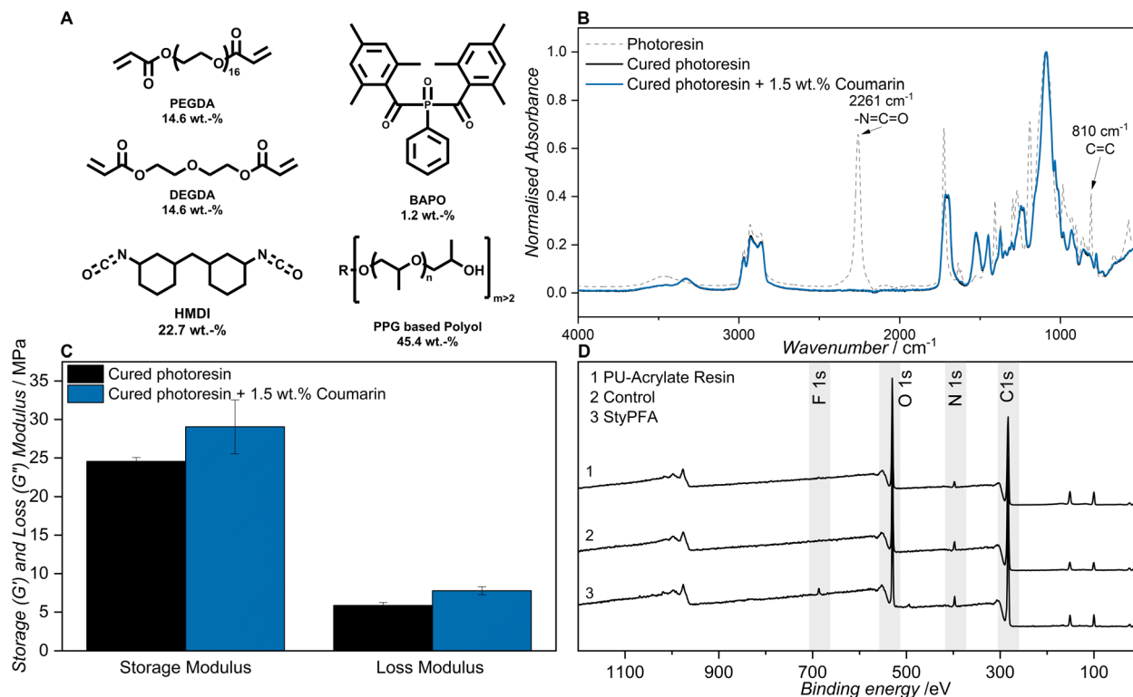
Fig. 3 (A) Components of the polyurethane–acrylate dual cure resin (B) FT-IR spectra overlayed of uncured resin (dashed grey) and cured 30 wt% resin (black) and 30 wt% resin with 1.5 wt% coumarin (blue) in the range from 400 to 4000 \text{cm}^{-1} . (C) Storage modulus ( G' ) and Loss modulus ( G'' ) measured at a frequency of 1 Hz of cured 30 wt% resin (black) and 30 wt% resin with 1.5 wt% coumarin (blue). (D) Wide scan XPS spectra of 1 freshly cured resin, 2 after the StyPFA treatment (2 \text{mmol L}^{-1} in ACN) in the dark and 3 after the StyPFA treatment under light (2 \text{mmol L}^{-1} in ACN under UVA and the emission spectrum of UVA lamps can be found in SI Section 1.2.7).
