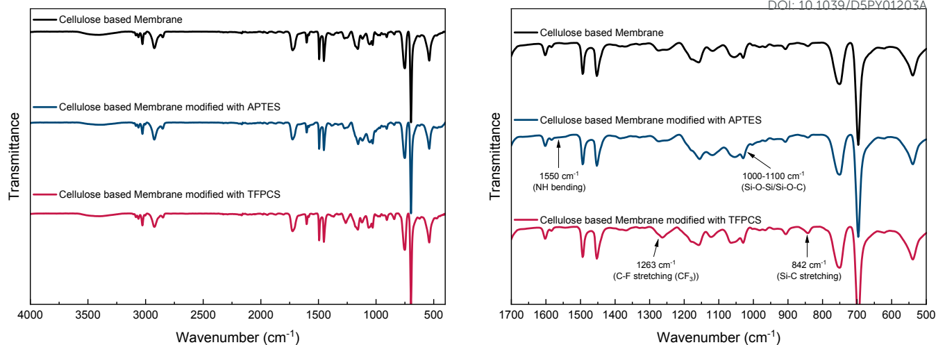
Figure 4: -FTIR spectra of the cellulose-based membrane coated with a porous structure based on PS-b-PDHPMA before post-modification (black), after ATPES modification (blue), and TFPCS modification (red). On the left side, an overview is given, while on the right, a detailed presentation is given.
