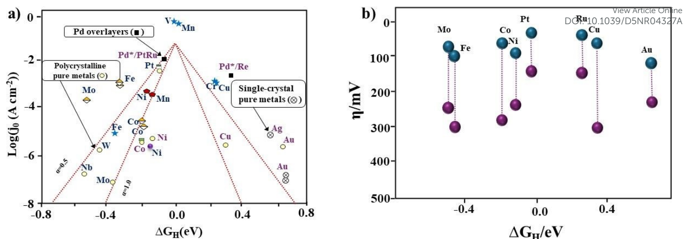
Figure 5. (a) Correlation between HER activity and hydrogen \Delta G_{H}^{*} for various metallic systems, including heteroatom-doped non-noble metal catalysts are represented. (b) The overpotential of non-noble metal catalysts doped with metallic heteroatoms is directly influenced by the \Delta G_{H}^{*} of the catalytic sites, which governs their hydrogen evolution efficiency.
