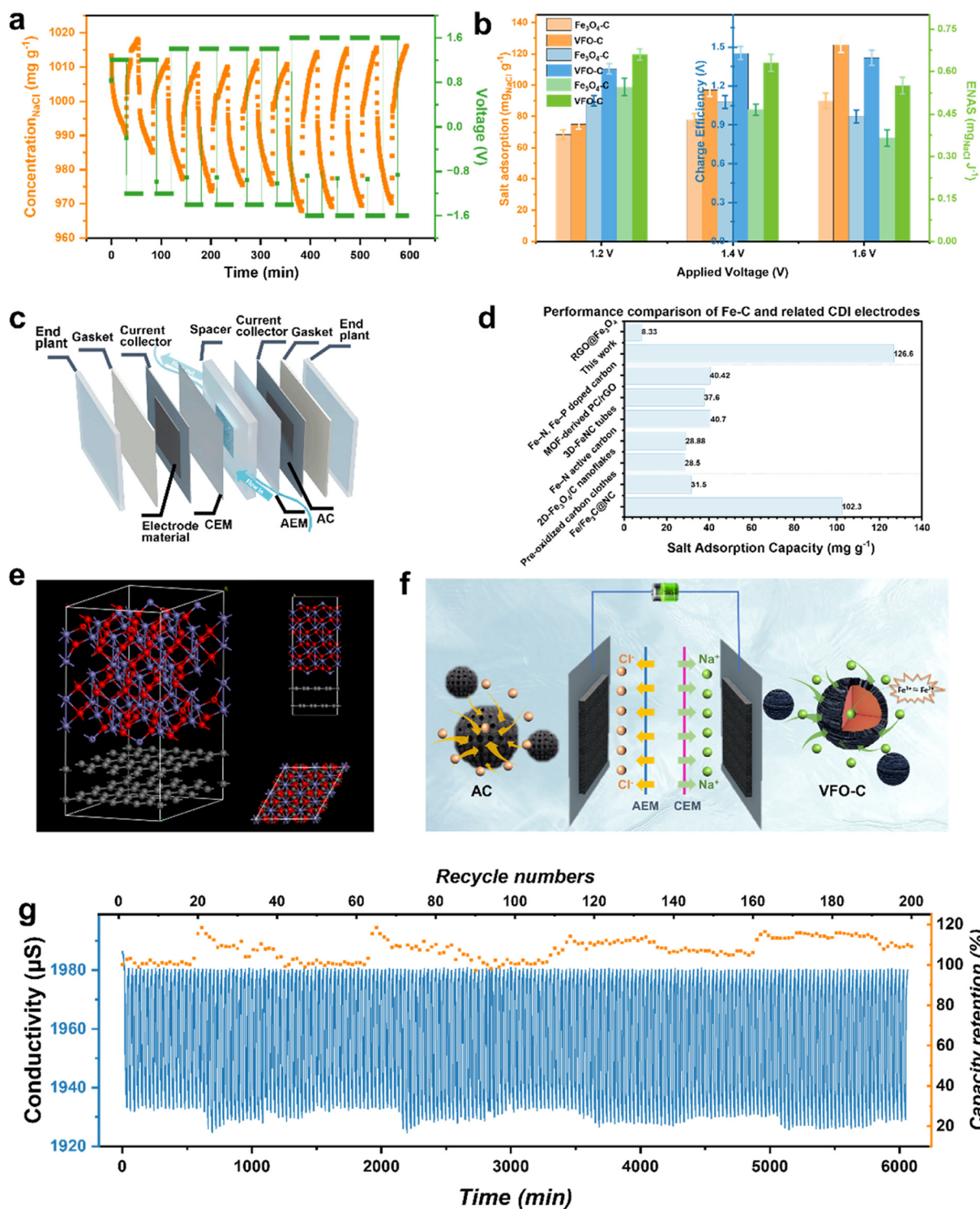
Fig. 4 (a) Concentrations responses of VFO-C electrode versus various cut-off voltage; (b) SACs, CEs and ENASs of VFO-C electrode and \text{Fe}_3\text{O}_4\text{-C} electrode at different cut-off voltages; (c) schematic illustrations of CDI devices; (d) performance comparison of VFO-C and related CDI electrodes; 50–57 (e) different perspectives on microstructure of VFO-C; (f) possible processes in both electrode materials during desalination; (g) the CDI cycling performances of VFO-C in 1000 \text{ mg L}^{-1} NaCl at 1.4 V.
