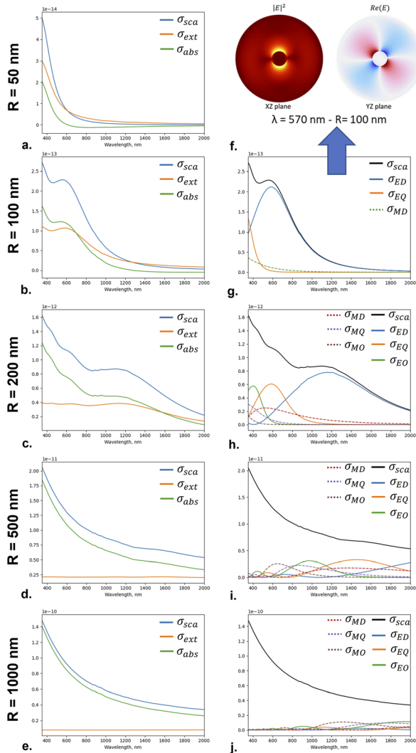
Fig. 6 Calculation of optical cross-sections and field distributions for HEA nanoparticles of different sizes. (a–e) Evolution of scattering ( \sigma_{\text{sca}} , blue), absorption ( \sigma_{\text{abs}} , green), and extinction ( \sigma_{\text{ext}} , orange) cross-sections for nanoparticles with radii of 50, 100, 200, 500, and 1000 nm, showing transitions from Rayleigh to Mie and then to geometrical scattering regimes. (f) Electric field distribution around a 100 nm radius nanoparticle at 570 nm wavelength in the XZ and YZ planes, revealing dipole-like behaviour. (g–j) Multipole decomposition of scattering cross-sections for nanoparticles of increasing size, showing contributions from various electric and magnetic modes (E: electric mode, M: magnetic mode, D: dipole, Q: quadrupole, O: octupole). (k) Temperature elevation of nanoparticles as a function of their radius and the incident wavelength for an incident power of I = 0.1 \mu\text{W} \mu\text{m}^{-2} .
