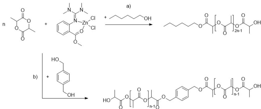
Scheme 1 Lactide ROP catalysed by [ZnCl 2 (TMGasme)] (C1) with two different co-initiators: (a) 1-hexanol (CoI1); (b) 1,4-benzenedimethanol (CoI2).
