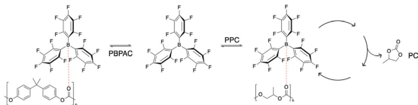
Scheme 1 Representation of possible interactions between BCF and carbonate groups for the depolymerization of PBPA and PPC mixture explaining slower CDP rates in the presence of two polycarbonates.
