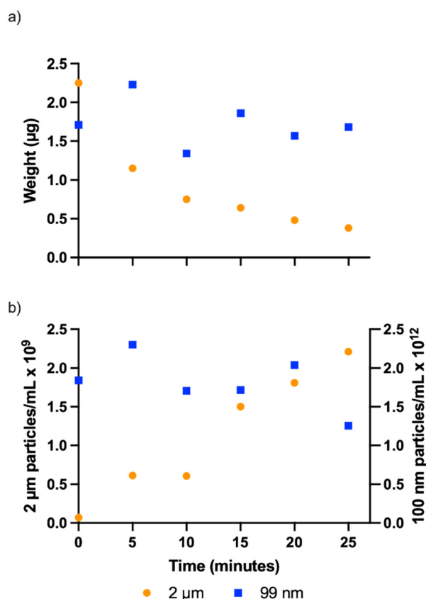
Fig. 5 Characteristics of the 2 μm and 99 nm polystyrene nanoparticles after mechanical breakdown. a. Estimated total weight calculated from DCS data for peaks around 100 and 1700 nm. b. Particle concentration of the small particles resulting from the mechanical breakdown of 2 μm polystyrene particles and the 99 nm particles estimated from NTA data. The data is from samples filtered through a 0.8 μm filter. The size of the 2 μm particles decreases with time (see Table S3).
