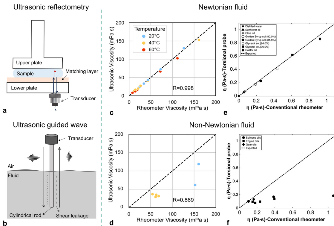
Fig. 11 Ultrasonic measurement approach for fluid viscosity. (a) An illustration of shear wave ultrasonic reflectometry (redrawn based on ref. 224); (b) a schematic of a guided wave measurement setup in torsional mode (redrawn based on ref. 228); (c) and (d) a comparison of viscosity measured from ultrasonic reflectometry and conventional rheometer for Newtonian-like lubricants and Non-Newtonian fluid respectively. Reproduced from ref. 224. Copyright 2024, licensed under CC BY 4.0, Elsevier Ltd. (e) and (f) A comparison of viscosity measured from conventional rheometer and the torsional waveguide probe for Newtonian fluid and Non-Newtonian fluid respectively. Reproduced from ref. 228. Copyright 2011, licensed under CC-BY-NC-ND 4.0, Institute of Electrical and Electronics Engineers.
