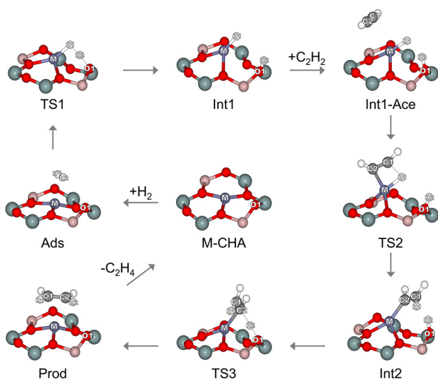
Fig. 2 Reaction mechanism for the acetylene hydrogenation to ethylene on M-CHA. Si, Al, O, C, H and metal atoms are represented in green, pink, red, grey, white, and blue, respectively.
