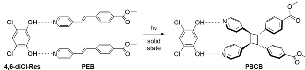
Scheme 2 The templated [2 + 2] photocycloaddition of PEB to afford PBCB .
