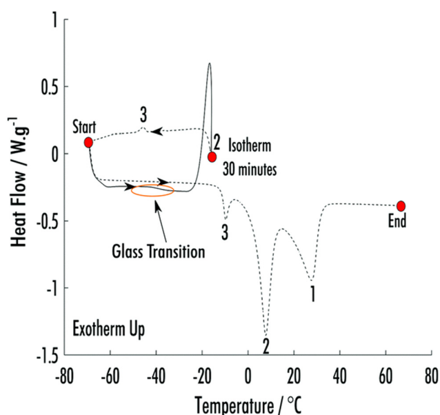
Fig. 2 DSC of an 8:1 phenol:2-ethoxybenzamide VODES. At the point “start” the sample has been cooled to -70\text{ }^{\circ}\text{C} from 70\text{ }^{\circ}\text{C} . The thermogram follows the solid line and then dashed lines. The numbers highlight the crystallisation and melts of the different phases. 3 is the phase formed on cooling the sample after it had been held at T_{c2} . 2 is the new phase that formed during synchrotron-DSC analysis. 1 is the ambient crystal structure of phenol, which had already crystallised during the initial cool from 70\text{ }^{\circ}\text{C} . Reprinted from ref. 8 with permission from C. L. Hall, J. Potticary, V. Hamilton, S. Gaisford, A. Buanz and S. R. Hall, Chem. Commun. , 2020, 56, 10726–10729. Copyright 2020 Royal Society of Chemistry.
