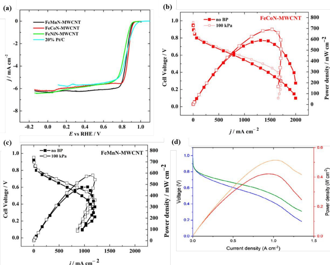
Fig. 9. (a) ORR polarization curves recorded in \text{O}_2 -saturated 0.1 \text{ M KOH} . AEMFC polarization and power density curves using (b) FeCoN-MWCNT and (c) FeMnN-MWCNT cathode catalysts. Reproduced from ref. 66 under a Creative Commons Attribution Licence (CC-BY), copyright 2021 the authors. (d) AEMFC performance using HT-FeCu porphyrrole aerogel-based cathode catalyst. Testing conditions: temperature 75/77/80^\circ \text{C} , \text{H}_2/\text{O}_2 , 150 \text{ sccm} . Performances with (green and orange) and without (blue and red) iR correction. Reproduced from ref. 137 under a Creative Commons Attribution Licence (CC-BY), copyright 2023 the authors.
