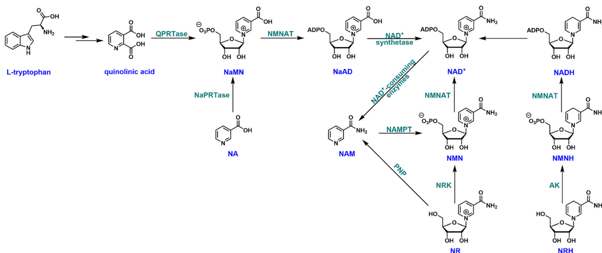
Fig. 1 \text{NAD}^+ biosynthetic pathways in mammalian cells.
