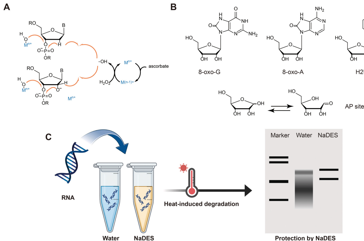
Fig. 2 Chemical factors and thermal stress that affect mRNA stability. (A) Summary of hydrolytic and oxidative cleavage pathways for nucleic acids, promoted by metal complexes. Reproduced with permission from ref. 49. Copyright 2018, Elsevier. (B) Structures of oxidative RNAs: 8-oxo-G (8-oxo-7,8-dihydro-guanosine), 8-oxo-A (8-oxo-7,8-dihydro-adenosine), H2U (4-pyrimidinone ribofuranoside), and AP site (apurinic/apyrimidinic site). Reproduced with permission from ref. 44. Copyright 2021, the Authors. (C) Natural deep eutectic solvents protect RNA from thermal-induced degradation. Reproduced with permission from ref. 50. Copyright 2023, Elsevier.
