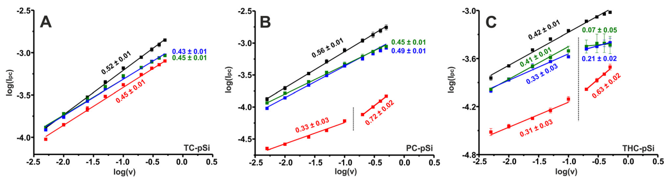
Fig. 5 \log(I_{pc}) vs. \log(\nu) plots with the corresponding slopes for (A) TC-pSi, (B) PC-pSi, and (C) THC-pSi. Coloured symbols indicate: black – bare electrode, red – at 24 h biofilm growth, blue – at 48 h biofilm growth, and green – at 72 h biofilm growth. Error bars represent the standard deviation of the measurements for three electrodes.
