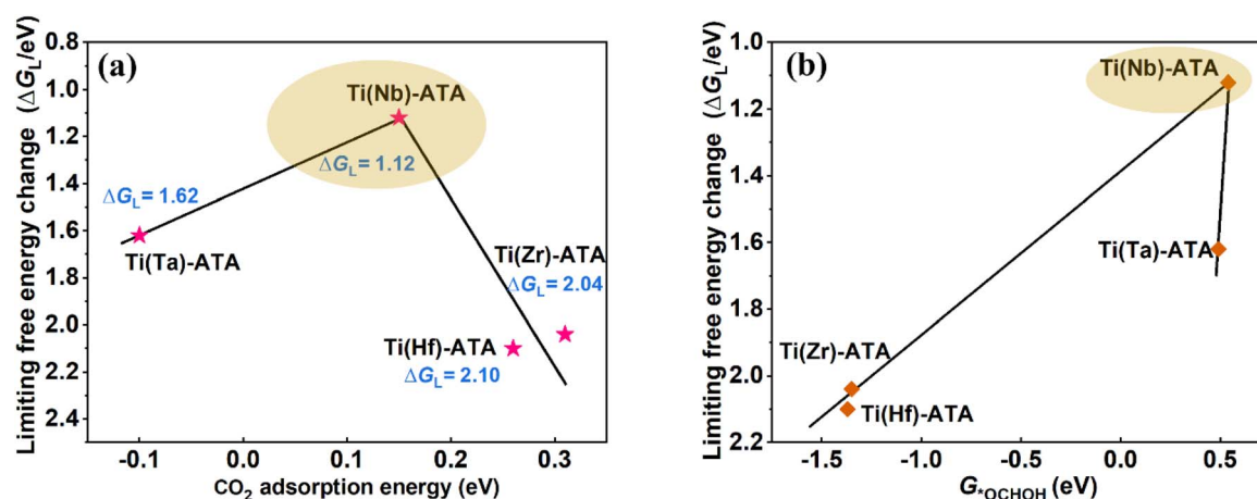
Fig. 6 Volcano-type curves between (a) CO 2 adsorption energy, (b) G_{*OCHOH} and limiting free energy change for C 2 products generation on Ti(M)-ATA (M = Zr, Hf, Nb, Ta) catalysts.
