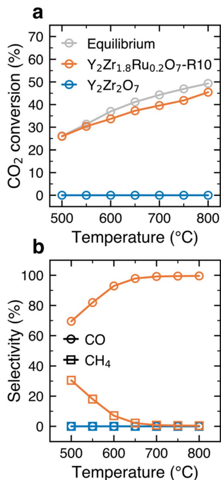
Fig. 9 Catalytic activity measurements of \text{Y}_2\text{Zr}_{1.8}\text{Ru}_{0.2}\text{O}_7\text{-R10} (reduced for 6 h at 1000 °C under flowing 5% \text{H}_2/\text{N}_2 , with a 5 \text{ °C min}^{-1} ramp rate) for the reverse water gas shift reaction. (a) The percentage of \text{CO}_2 converted compared against equilibrium, and (b) the selectivity of conversion to CO and \text{CH}_4 , as a function of temperature.
