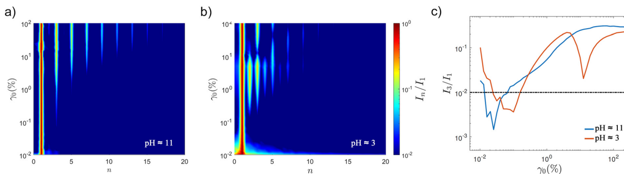
Fig. 10 (a) and (b) FT maps of higher harmonics ( n ) for STO formulations before and after triggering the assembly using HCl, at pH values ≈11 and 3 respectively. The aggregated STO formulation has intense even harmonics and non-linearities at small strain amplitudes. (c) The evolution of the relative intensity of the third w.r.t. the first harmonic ( I_3/I_1 ) shows distinctive trends for the two samples.
