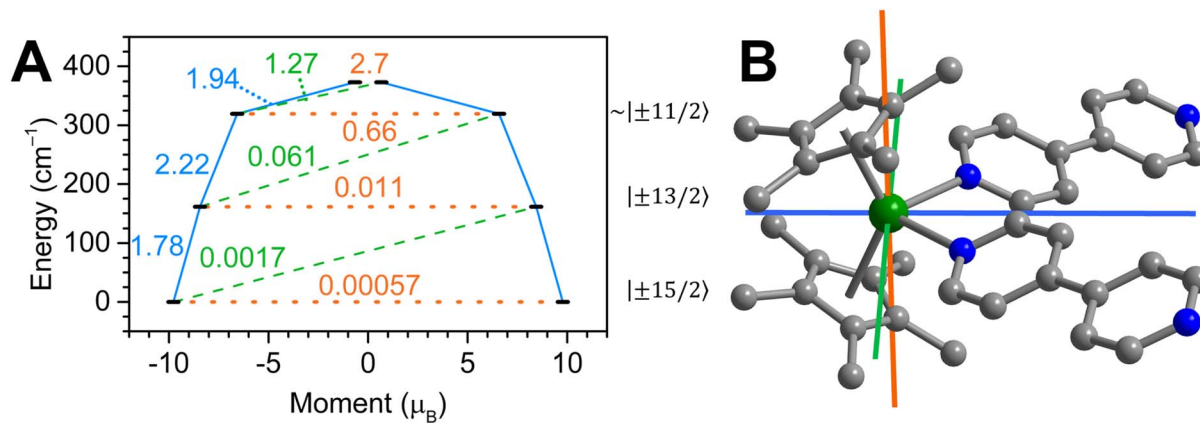
Fig. 8 (A) Estimated relaxation barrier comprising the four lowest-lying Kramer's doublets with relaxation pathways shown for [\text{Cp}_2^*\text{Dy}(\text{bpy})_2]^+ , 3' . Solid blue and dashed green lines indicate Orbach relaxation processes, orange dotted lines indicate quantum tunnelling of the magnetisation (QTM)/thermally activated QTM pathways. Values next to the arrows correspond to the respective transition magnetic moment matrix elements. The numbers on the right are given for the primary M_J state comprising the wave function for each state. (B) Plot of the g -tensor components calculated for the |\pm 15/2\rangle ground state Kramer's doublet of 3' . Colour code: g_x (green), g_y (blue) and g_z (orange) with respective compositions 0.0007 ( g_x ), 0.0027 ( g_y ) and 19.5595 ( g_z ).
