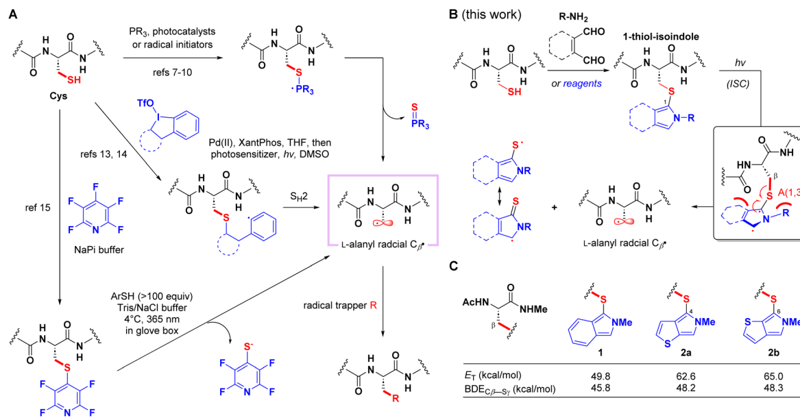
Fig. 1 Previous methods for radical desulfurative modifications of cysteine and the approach proposed in this study. (A) Phosphine-assisted desulfuration via phosphoranil radicals, S H2 strategy, and thiol activation through photoinduced electron transfer to fluoropyridines. (B) The postulated photo-induced C β -S bond homolysis based on the isoindole chromophore. (C) DFT calculations of three different chromophores; energy obtained at the (U)ωB97X-D/def2 TZVP/SMD(H 2 O)//(U)ωB97X-D/def2-SVP/SMD(H 2 O) level.
