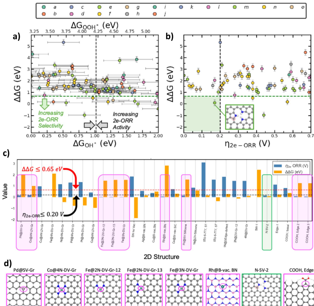
Fig. 4 (a) Selectivity analysis showing \Delta\Delta G as a function of \Delta G_{\text{OOH}}^* for various investigated active sites in carbon-based materials and two-dimensional boron nitride. (b) Combined selectivity-activity map, where the highlighted green region indicates the optimal zone for both high selectivity and catalytic activity. The inset displays the atomic structure and highlights the active site (indicated by red circles) of the only structure that meets both the high activity and selectivity criteria. Labels a to j correspond to the reported values on various two-dimensional materials in the literature as reported in the SI. Error bars on data points show the individual uncertainties in each datapoint. (c) Bar chart highlighting the most promising two-dimensional structures exhibiting either \Delta\Delta G \leq 0.65 eV (indicated by the red dashed line) or \eta_{2e-ORR} \leq 0.20 V (indicated by the black dashed line). (d) Several examples of the atomic structures highlighted in pink and green in the bar chart. Red oval indicates the active site.
