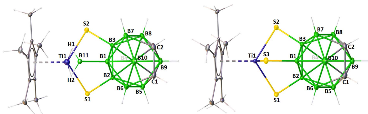
Fig. 5 Molecular structure and labelling diagram of 3 (left) and 4a (right). Selected bond lengths ( \text{\AA} ) and bond angles ( ^\circ ): 3 : Ti1-S1 2.3321(9), Ti1-S2 2.3214(9), Ti1 \cdots B11 2.259(4), Ti1-H1 2.00(3), Ti-H2 1.93(3), B11-H1 0.90(3), B11-H2 1.03(4), B1-B11 1.750(5), B2-S1 1.851(4), C1-C2 1.626(6), Ti1-S1-B2 81.17(11), B2-B1-B11 121.9(3). 4a : Ti1-S1 2.3095(12), Ti1-S3 2.3231(12), B1-S3 1.849(5), B1-B2 1.829(5), C1-C2 1.635(7), C1-B10 1.713(7), Ti1-S1-B2 80.72(14).
