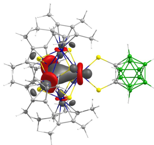
Fig. 4 HOMO of 2 showing 3c–2e equatorial trititanium interactions (isocontour values: ±0.045 [e bohr –3 ] 1/2 ).
