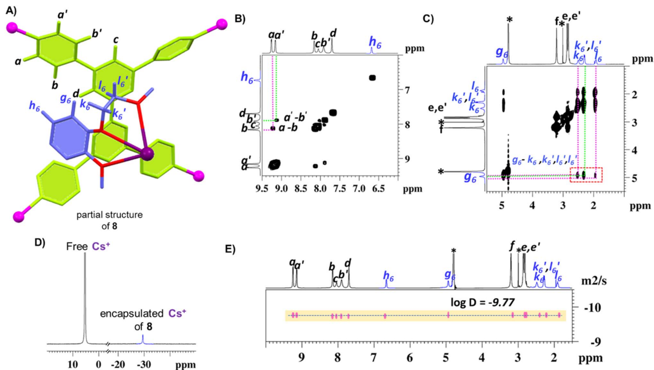
Fig. 7 (A) Partial representation of [(\text{G}\subset(\text{H6})_2)\subset\text{H1}]\cdot 17\text{NO}_3 , 8 , showing one of the walls of the super-host and part of the encapsulated host-guest complex. (B and C) Partial ^1\text{H} - ^1\text{H} COSY and ^1\text{H} - ^1\text{H} NOE spectra (400 MHz, \text{D}_2\text{O} , 298 K) emphasising correlations between certain protons (for COSY: a with b and a' with b'; for NOE: g_6 with k_6 , k'_6 , l_6 , and l'_6 ) for characterization of 8 . (D) ^{133}\text{Cs} NMR spectrum (66 MHz, \text{D}_2\text{O} , 298 K) of 8 in the presence of excess \text{Cs}^+ , supporting the encapsulation of G, i.e., \text{Cs}^+ . (E) ^1\text{H} -DOSY NMR spectrum (500 MHz, \text{D}_2\text{O} , 298 K) of 8 showing a single band for which the calculated diffusion coefficient ( D ) value is 1.67 \times 10^{-10} \text{ m}^2 \text{ s}^{-1} .
