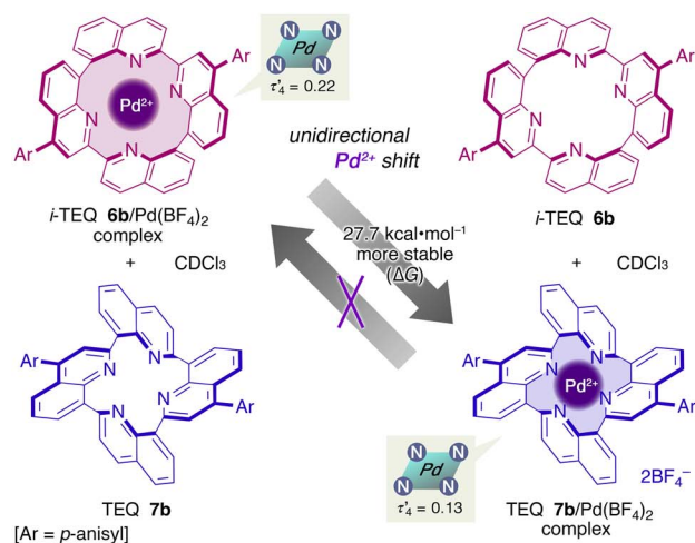
Scheme 3 Unidirectional Pd 2+ cation swapping between i -TEQ 6b and TEQ 7b . Partial 1 H NMR spectra in CDCl 3 (i) i -TEQ 6b /Pd(BF 4 ) 2 ; (ii) TEQ 7b ; (iii) i -TEQ 6b /Pd(BF 4 ) 2 + TEQ 7b at reflux temperature after 4 h; (iv) i -TEQ 6b ; (v) TEQ 7b /Pd(BF 4 ) 2 ; (vi) TEQ 7b /Pd(BF 4 ) 2 + i -TEQ 6b at reflux temperature after 4 h.
