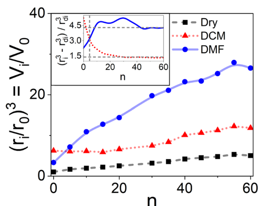
Fig. 4 Average relative volume (r_i/r_0)^3 for the solid support (1% cross-linking, 0.95 mmol \text{g}^{-1} ) relation with the number of repeating units ( n ) from i = 0 to i = n . Dry beads (black squares), compared to swollen particles in DCM (red triangles) and DMF (blue circles); based on the experimental data from Sarin et al. 28 (Table III). In all cases, r_0 refers to the dry original bead. The insert depicts the relative solvent volume increase [(r_i^3 - r_d^3)/r_d^3] comparing the swollen volume to the dry state r_d (red dotted line for DCM and blue continuous line for DMF).
