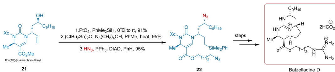
Scheme 11 Evans' synthesis of tricyclic guanidine alkaloids-batzelladine D.
