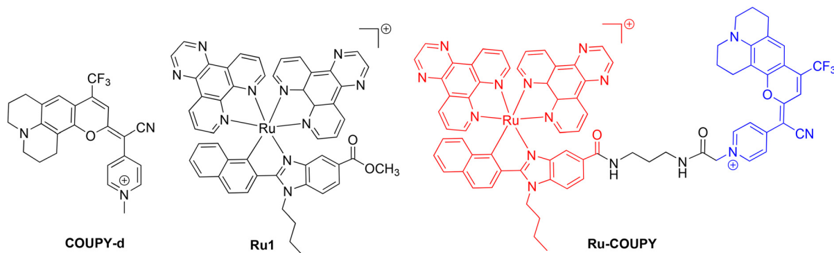
Fig. 6 Structure of Ru(II)-COUPY conjugate and of the parent coumarin and Ru(II) complex.
