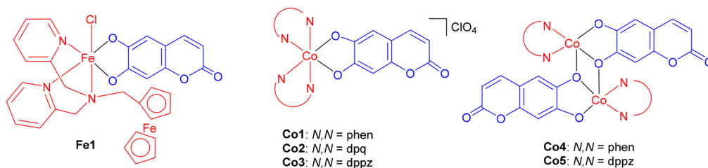
Fig. 10 Earth-abundant metal PSs with coumarin directly coordinated as O^{\wedge}N ligand.
