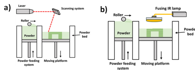
Fig. 11 Schematics of 3D printing techniques (a) SLS, and (b) MJF. Reproduced with permission from ref. 108. Copyright 2022, Elsevier.
