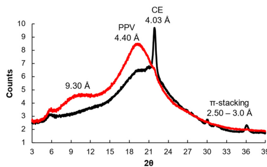
Fig. 5 WAXS diffractograms corresponding to homopolymer CE-PPV ( 13b ) (black) and the supramolecular bottlebrush CE-PPV-PS-DBA + (red).
