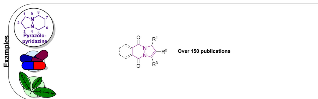
Fig. 6 Examples of various pyrazolo-pyridazine-derived compounds.
