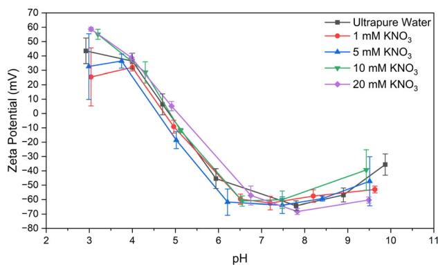
Fig. 6 Zeta potential of BSA nanoparticles synthesized in several different concentrations of KNO 3 , all washed and redispersed in 1 mM KNO 3 ( n = 3 for each electrolytic strength). Regardless of electrolytic strength during synthesis, zeta potential of the washed dispersion was effectively unchanged, and the isoelectric point remained similar to that of naked albumin.
