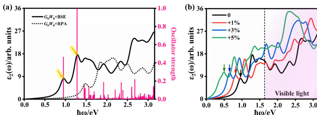
Fig. 8 (a) Imaginary part ( \varepsilon_2 ) of the dielectric function of the pristine AA5 GaN/MoSi 2 P 4 heterobilayer is calculated with (black solid line) and without (black short dash line) electron–hole coupling included, i.e. , G_0W_0 +BSE and G_0W_0 +RPA, respectively. (b) \varepsilon_2 of the GaN/MoSi 2 P 4 heterobilayer at biaxial tensile strains of +1%, +3%, and +5% using the G_0W_0 +BSE method. The incident polarized light is along the x direction. A Lorentzian broadening of 100 meV is applied in these calculations.
