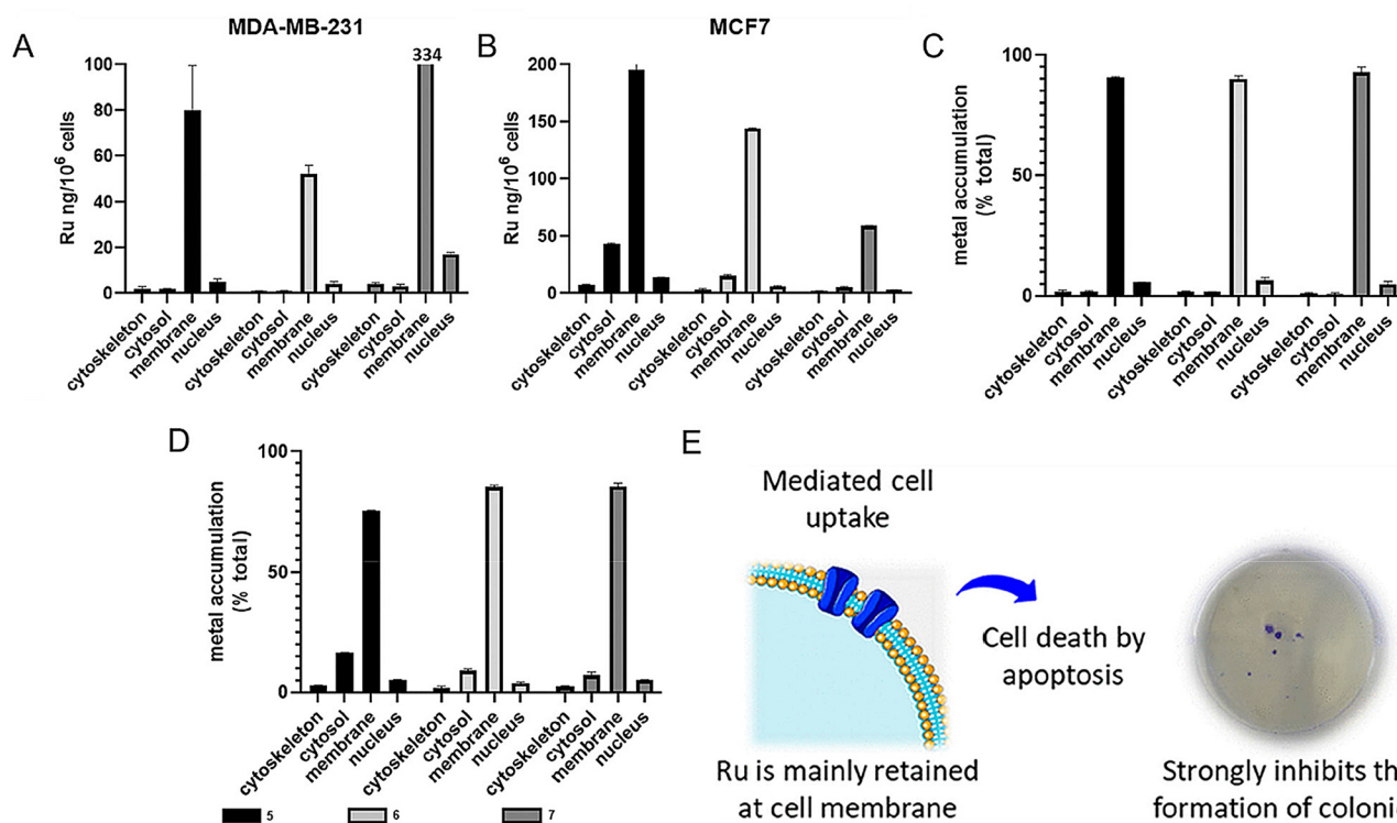
Fig. 6 Chemical structures of compounds 4 , 5 and 6 . ( A–D ) Distribution of Ru in cells after drug treatment. ( E ) Representative images of colony formation assay. Reproduced with permission. 39 Copyright 2019, ACS.
