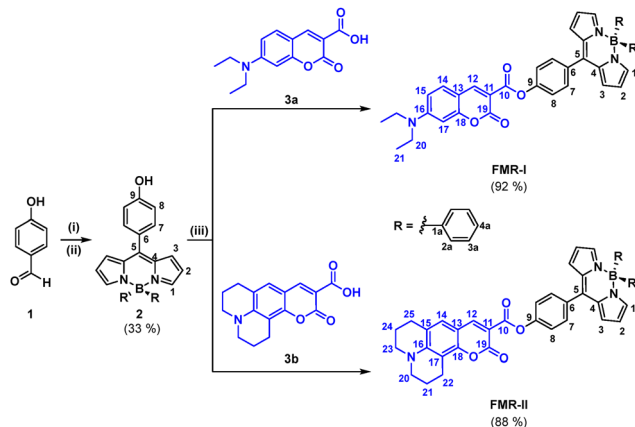
Scheme 2 Synthesis and numbering of fluorescent molecular rotors FMR-I and FMR-II . Reagents and conditions: (i) Pyrrole, TFA, DCM, rt; (ii) DDQ, diphenylboronic acid, THF, reflux; (iii) DCC, DMAP, DCM, microwave irradiation (100 W, 80 °C).
