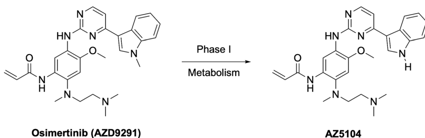
Fig. 3 AZ5104 is a phase I metabolite of osimertinib and associated with dose-limiting adverse events.
